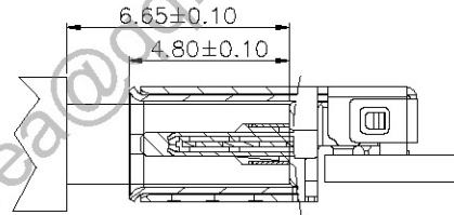
MATED CONDITION(REF.)
