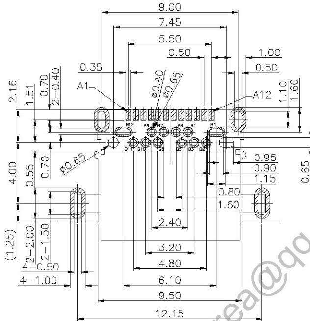
RECOMMENDED P.C.B. LAYOUT TOLERANCE UNSPECIFIED \pm 0.05\text{mm} (TOP VIEW)
