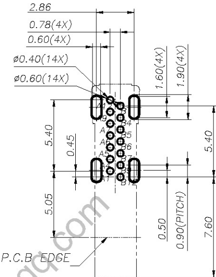
RECOMMENDED PCB LAYOUT(TOP VIEW) THICKNESS 1.6±0.10MM;DEFAULT TOLERANCE:±0.05
