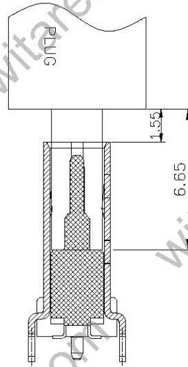
AFTER MATING
