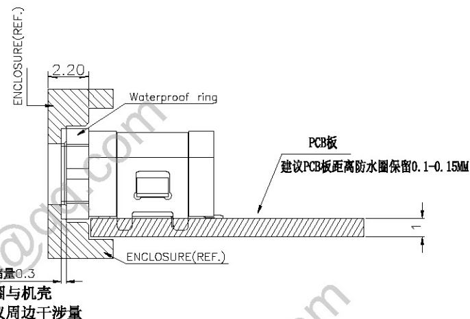
RECOMMENDED SCHEMATIC DRAWING OF CONNECTOR MATCH CHASSIS
